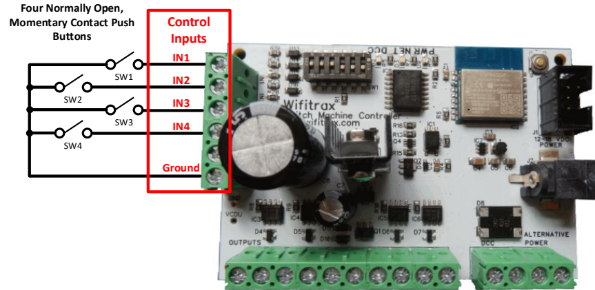
Figure 5. Connection Diagram for Manual Push Buttons
