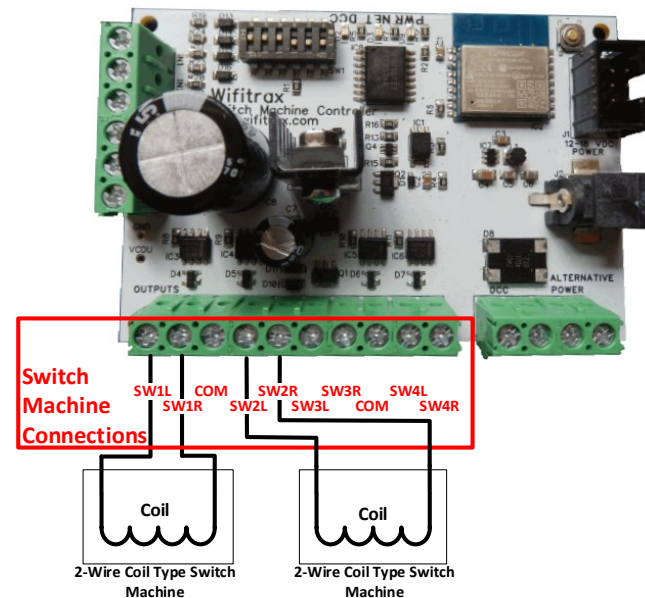
Figure 3. Connection Diagram for 2-Wire Coil-Type Switch Machines
