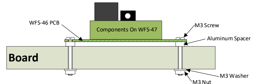
Figure 6 Mounting Suggestion
