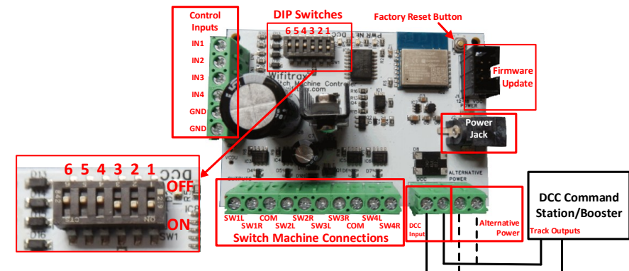
Figure 1 WFS-47 Connections
