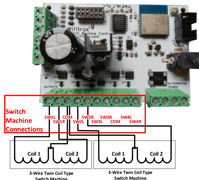
Figure 2. Connection Diagram for 3-Wire Twin Coil Switch Machines
