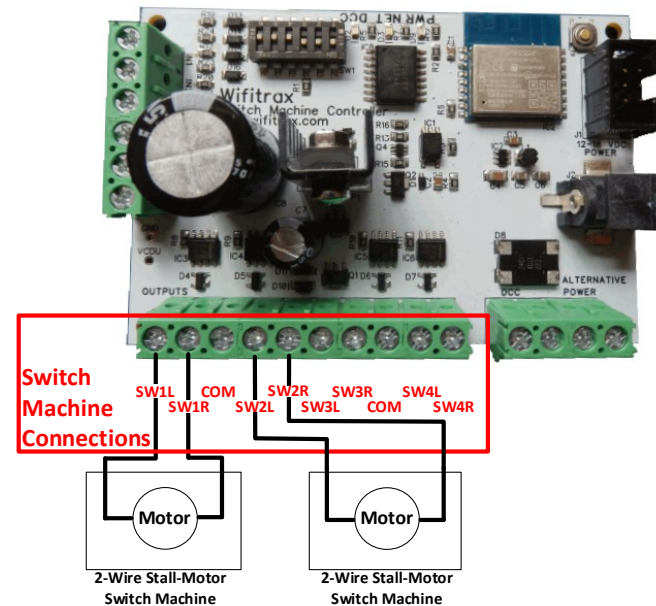
Figure 4. Connection Diagram for Stall Motor Switch Machines
